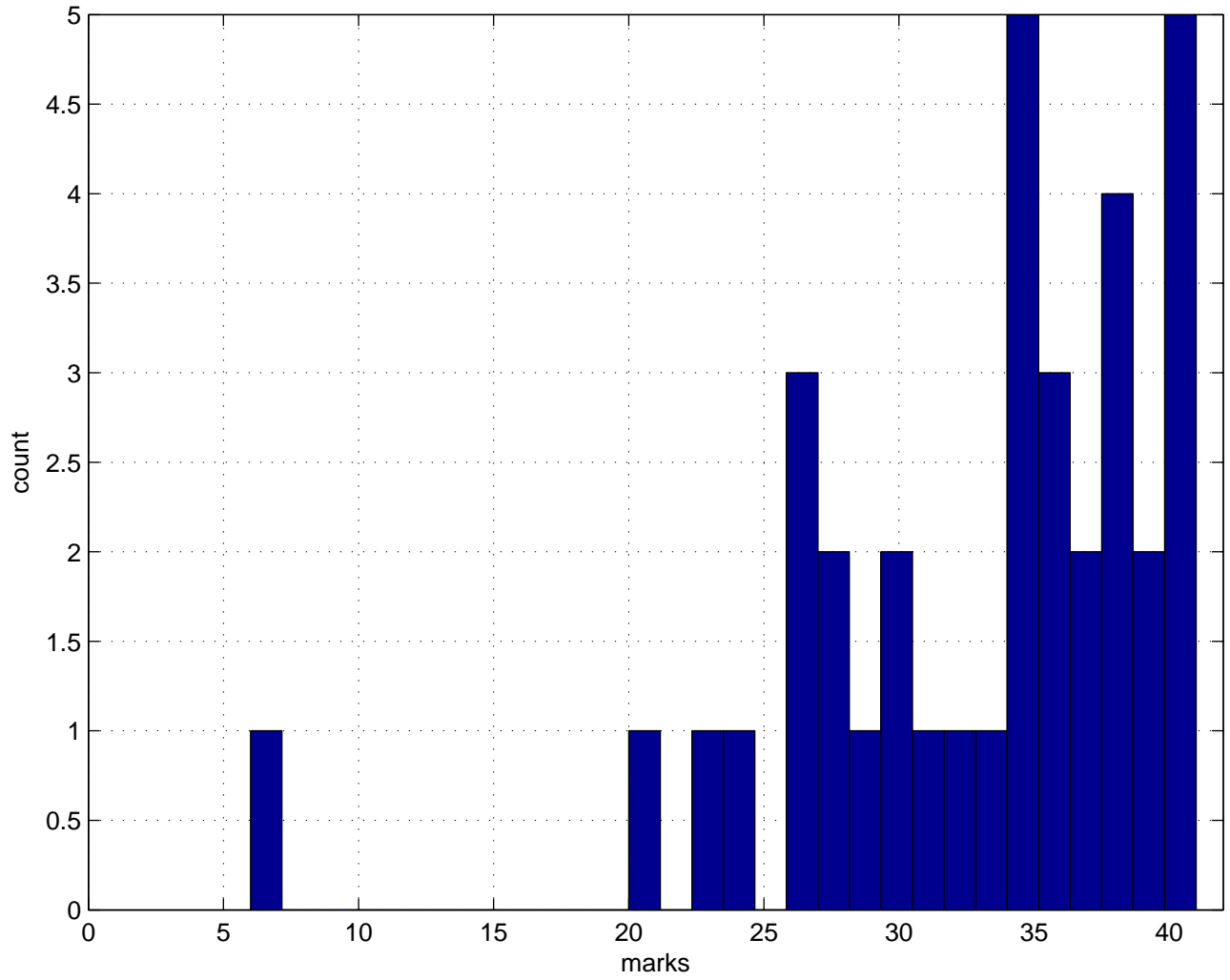
Midterm 2010 – Histogram
