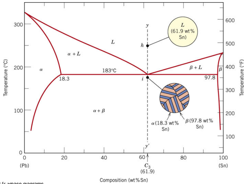
Chapter 9: Phase diagrams
