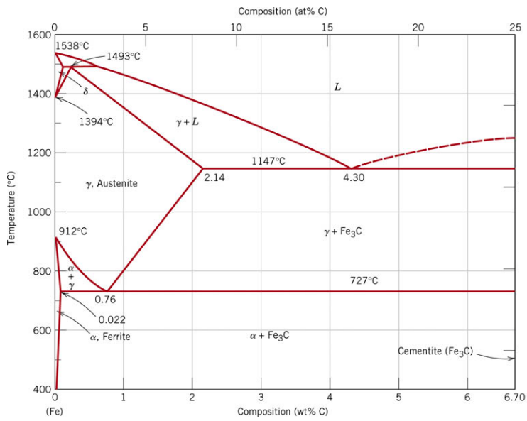
Chapter 9: Phase diagrams
