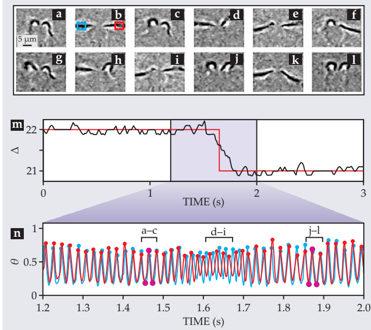
Figure 2. Phase slip. The two flagella that emerge from the alga Chlamydomonas reinhardtii usually mirror each other with near-perfect synchrony. But in an occurrence known as a phase slip, the flagella transition from a phase-locked state (a–c) to an asynchronous state (d–i) and into a new phase-locked state (j–l). Time plots of experimental data (m,n) show that the phase slip, which occurs in just a fraction of a second, manifests as an integer jump in the flagella’s relative phase \Delta = (\theta_1 - \theta_2)/2\pi , where \theta_1 and \theta_2 are the phases of the points indicated by the blue and red boxes in panel b. (Adapted from ref. 3.)
