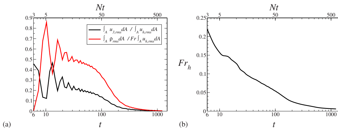
FIG. 16. (Color online) (a) Fluctuation strength. (b) Local horizontal Froude number. Both plots show data from the Pr=1 case, the same trends occur in all three cases.
