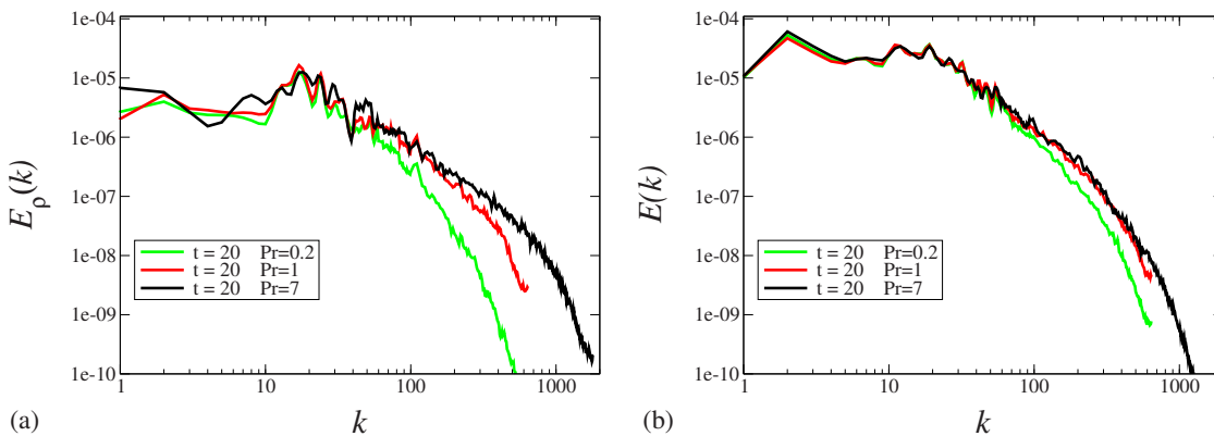
FIG. 12. (Color online) Separation in scales at different values of Pr. (a) E_\rho(k) . (b) E(k) .
