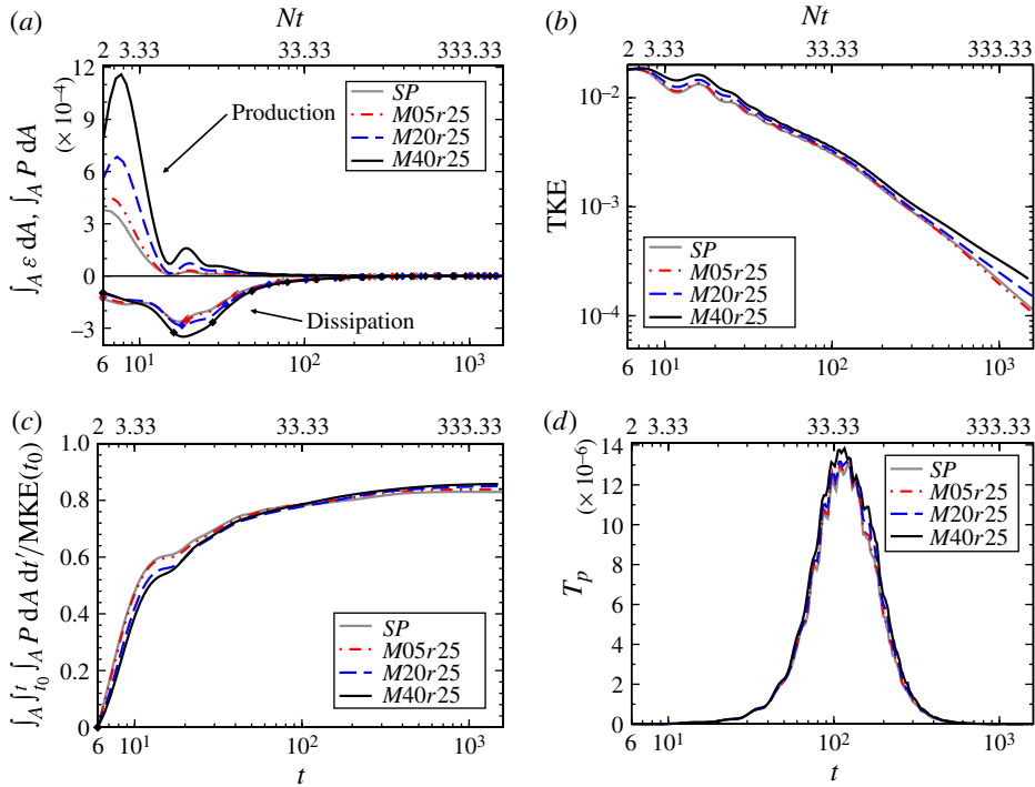
FIGURE 8. (Colour online) Effect of excess momentum on turbulent quantities: (a) integrated production and dissipation; (b) integrated turbulent kinetic energy; (c) cumulative integral of production normalized by initial MKE; (d) internal wave flux.
